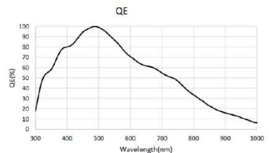
MV-CU020-80GM
