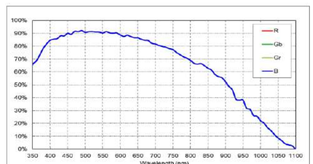
MV-CS050-60GM/GN
